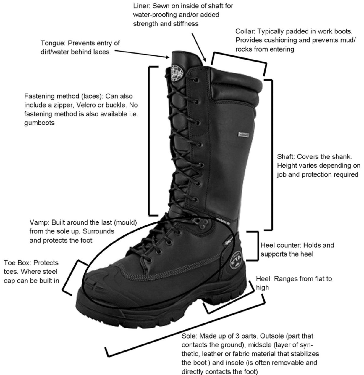
Fig. 1. Distinct design features of work boots (adapted from hotboots.com/bootinfo/terms.html and oliver.com.au).
